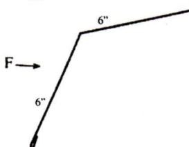
㉑ Gambrel Flash 10'
